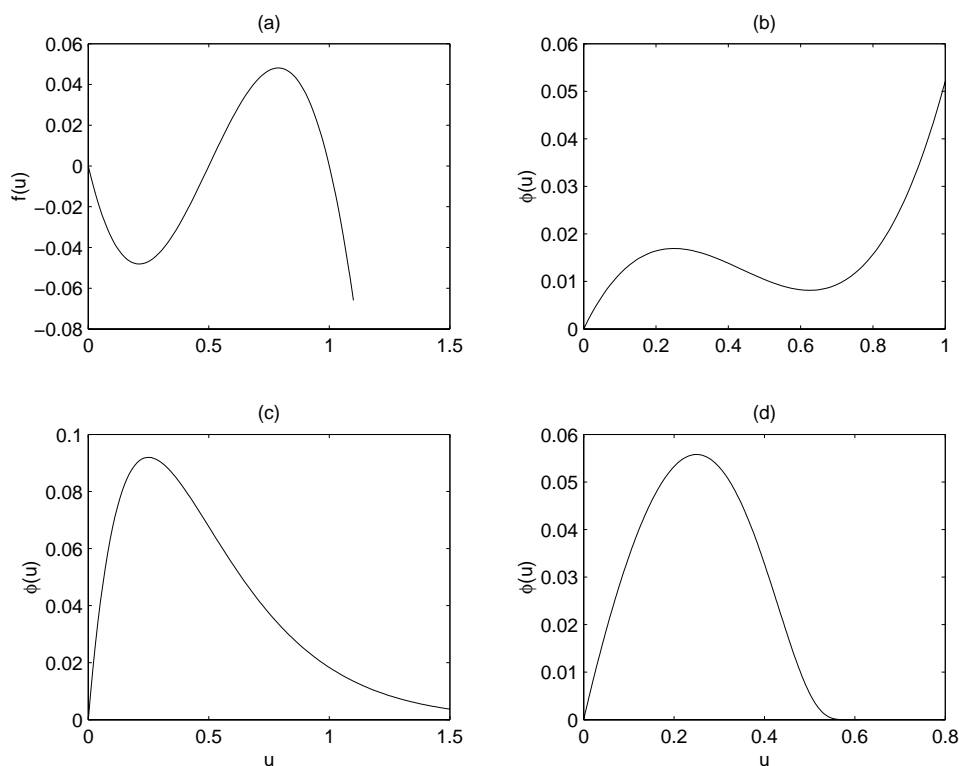
FIGURE 1. (a) f(u) = u(u-a)(b-u) , with a = 1/2 and b = 1 ; (b) \phi(u) = (u^3/3 - (\alpha + \beta)u^2/2 + \alpha\beta u) , with \alpha = 1/4 and \beta = 5/8 ; (c) \phi(u) = ue^{-\frac{u}{\alpha}} , with \alpha = 1/4 ; (d) \phi(u) = u \exp \frac{(\beta-\alpha)^2}{\alpha(u-\beta)} if 0 \leq u < \beta and \phi(u) = 0 if u \geq \beta , with \alpha = 1/4 and \beta = 5/8 .
